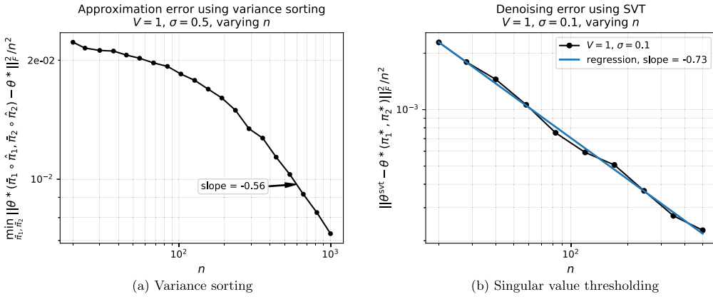
Figure 3. Algorithms for denoising pre-anti-Monge matrix. When an arrow is present, “slope” indicates the slope between two consecutive points.
