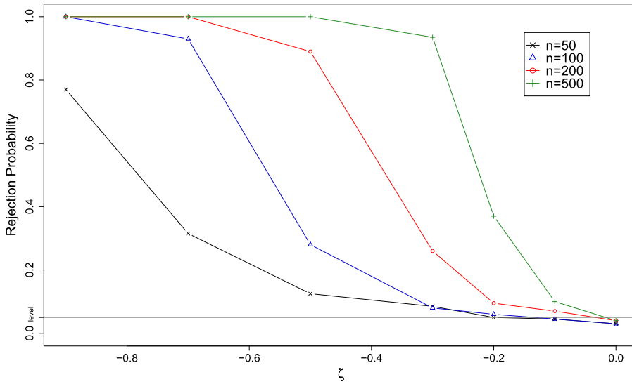
Figure 3. Monte-Carlo simulations for Example 4.1.
