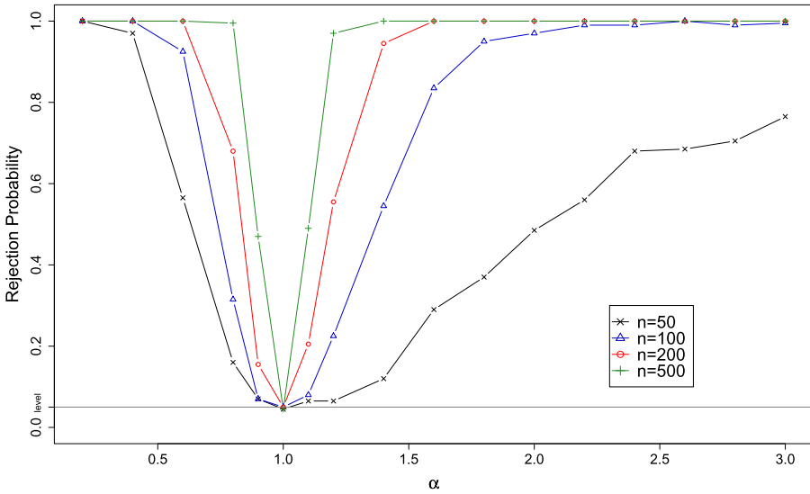
Figure 4. Monte-Carlo simulations for Example 4.2.
