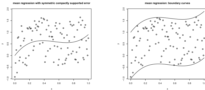
Figure 2. Example for data as in Remark 2.6.
