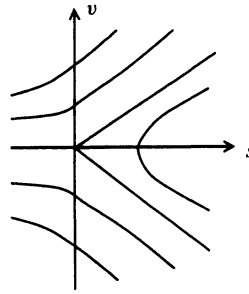
FIGURE 5.b. \varphi^*(\mathcal{F}_{2,\alpha}) .
