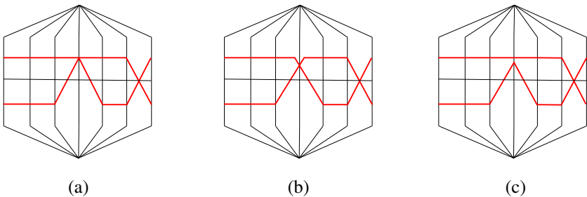
Figure 4: Normal coordinates drawn (a) without specifying gluings, (b) with a specified gluing, (c) with the opposite gluing from (b).
