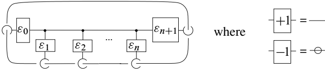
Figure 5. Here, a \ominus on an edge represents a negative half-twist.
