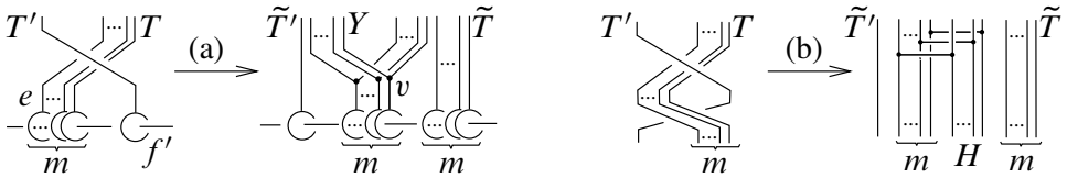
Figure 3. Leaf slide and crossing change involving parallel tree claspers
