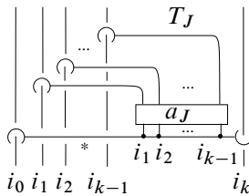
Figure 7. The C_k -trees T_J and \bar{T}_J
