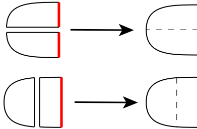
Figure 24: Module composition (top), n -category action (bottom)
