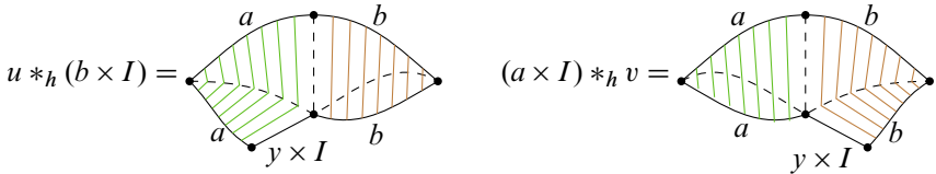
Figure 57: Horizontal compositions in the triangle axiom
