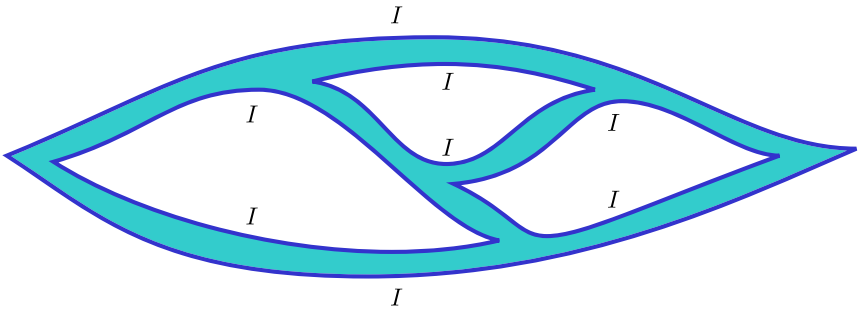
Figure 43: Little bigons, thought of as encoding surgeries
