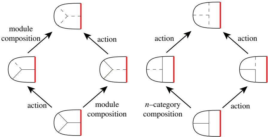
Figure 25: Two examples of mixed associativity
