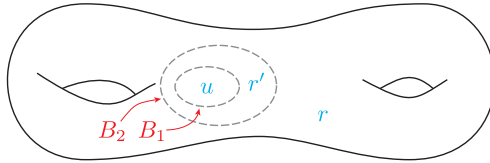
Figure 5: A nested 2–blob diagram
