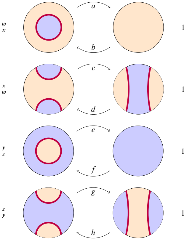
Figure 39: Intertwiners for a Morita equivalence
