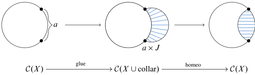
Figure 19: Extended homeomorphism
