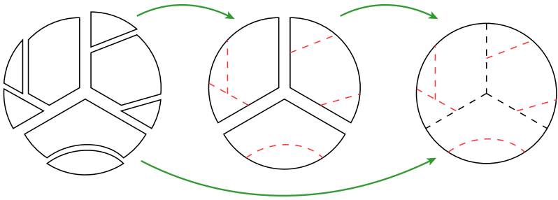
Figure 16: Operad composition and associativity
