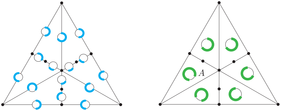
Figure 11: The 1- and 2-chains in the image of m \otimes a \otimes b . Only the supports of the blobs are shown, but see Figure 12 for an example of a 2-cell label.
