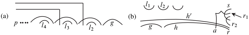
Figure 13. (a) The l_i flip to the other side of a leaf nonseparated from g (b) Convex neighborhood disjoint from all
