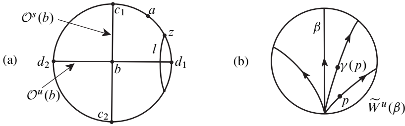
Figure 16. (a) The action of \gamma in \mathcal{D} and \partial\mathcal{O} . (b) Action of \gamma in \tilde{W}^u(\beta)
