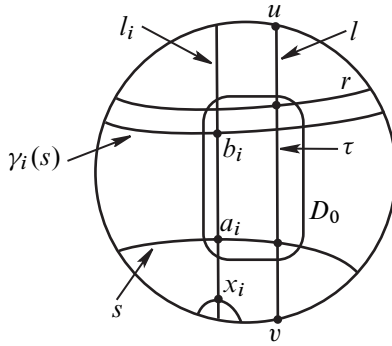
Figure 18. The case when \gamma_i(s) converges to a leaf r
