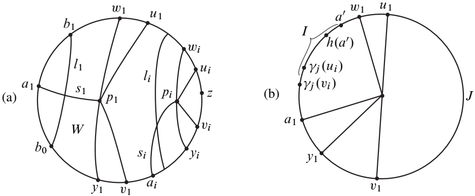
Figure 21. (a) Splitting in the stable leaves (b) Mapping back to a compact region
