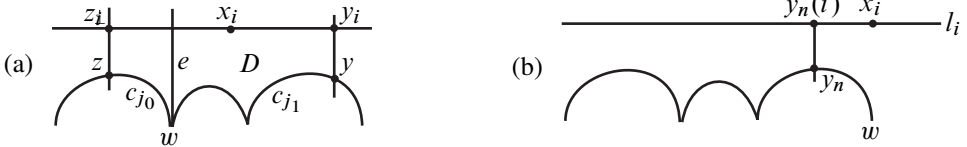
Figure 14. (a) The case that x_i is between some unstable leaves (b) The case that x_i escapes to one side
