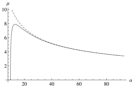
Figure 1. Numerical graph of \alpha \mapsto \mu(\alpha) in the supercritical case N = 3 and p = 3 (continuous line) and of the map \alpha \mapsto \alpha^{-1/2} \cdot \sqrt{3} \int_{\mathbb{R}^3} Z_{3,3}^2 dx (dashed line). The latter is the theoretical asymptotic expansion of \mu(\alpha) as \alpha \rightarrow +\infty as predicted by Lemmas 4.4 and 4.5.
