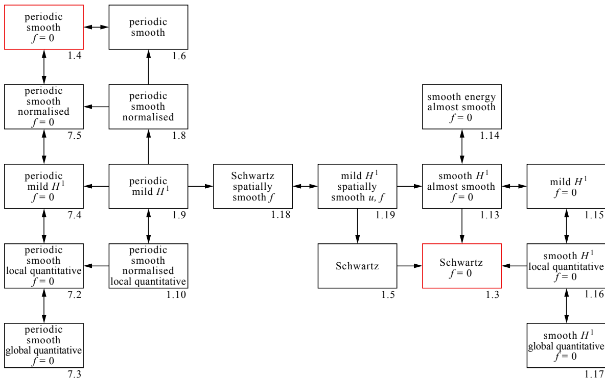
Figure 1. Known implications between the various conjectures described here (existence of smooth or mild solutions, or local or global quantitative bounds in the periodic, Schwartz, H^1 , or finite energy categories, with or without normalised pressure, and with or without the f = 0 condition) and also in [Tao 2007] (the latter conjectures and implications occupy the far left column). A positive solution to the red problems, or a negative solution to the blue problems, qualify for the Clay Millennium prize, as stated in [Fefferman 2006].
