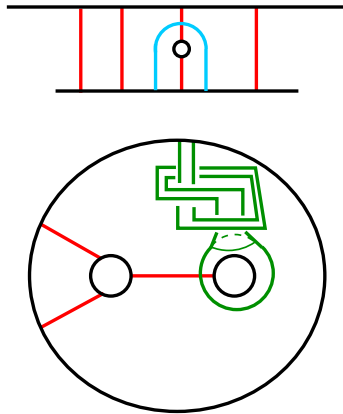
Figure 5: Above is an example of a vp-compressionbody (C, T) where \partial_-C has a semicut disc (shown in blue). Below is an example of an sc-disc with the property that boundary-reducing the vp-compressionbody along that disc does not result in the union of vp-compressionbodies.
