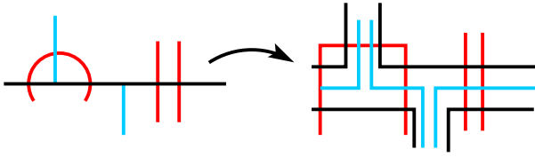
Figure 10: Untelesoping H . The red curves are portions of T . The blue lines on the left are sc-discs for H . Note that if a semicut or cut disc is used then a ghost arc is created.
