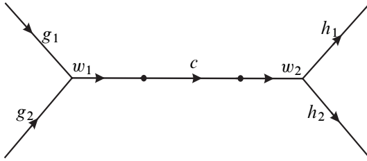
Figure 10: Construction of a \in H_2(N_\Gamma, \partial N_\Gamma)
