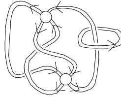
Figure 2: Singular framed link with 2 singularities
