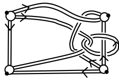
Figure 1: An example of a 3-web
