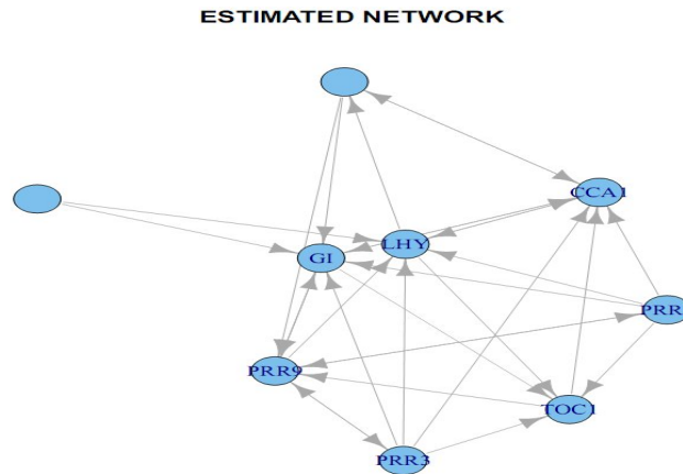
Fig. 5. Reverse genetic approach on Arabidopsis thaliana clock. Nodes refers to genes expression while empty nodes indicates latent variables in the form TFs.
