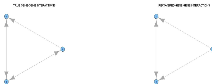
Fig. 3. Gene-gene interactions ZA + B . The true network(left) and the estimated network(right)
