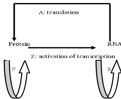
Fig. 1. Biological interpretation of the input SSM.
