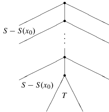
Figure 1 The tree S_n .
