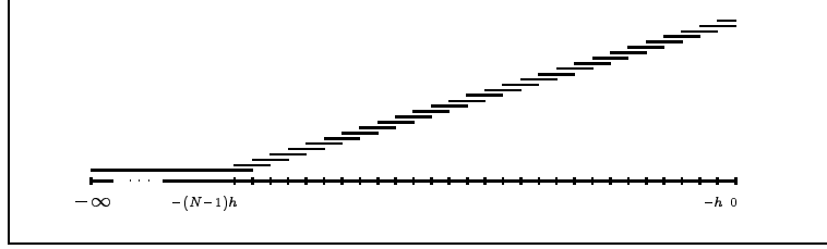
FIGURE 2. Supports of the functions \varphi_k over [-\infty, 0] .
