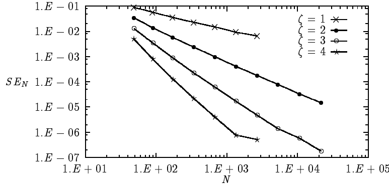
FIGURE 4. Orders of convergence.
