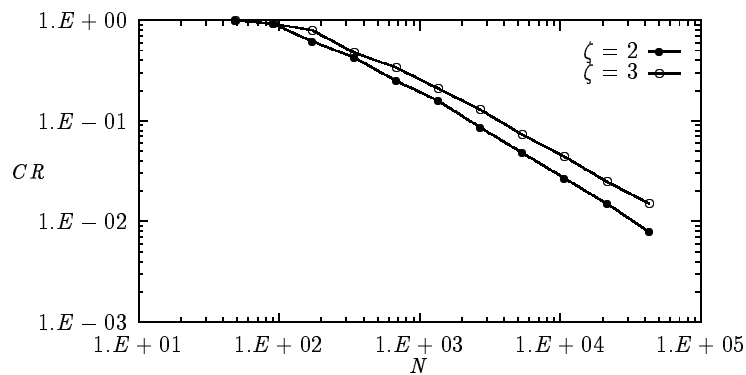
FIGURE 5. Compression rates.
