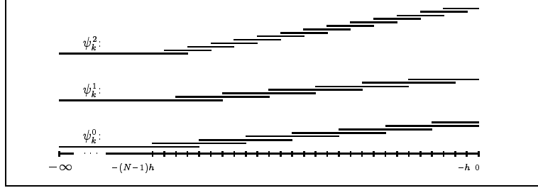
FIGURE 3. Supports of the functions \psi_k^l over [-\infty, 0] .
