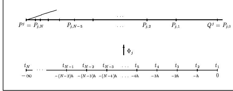
FIGURE 1. Grid points on (-\infty, 0] and \Gamma .
