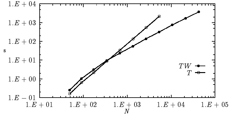
FIGURE 6. Time for the computation of the matrix in CPU-seconds, \zeta = 2 .
