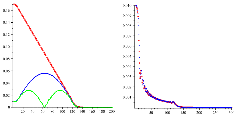
FIGURE 3.1. On the left, absolute values of A_{2n,2n} (boxes, the straight decreasing line), A_{2n,2n+2} (discs, the line with a single maximum) and A_{2n,2n+4} (points, the line with two maxima) and, on the right, absolute values of A_{0,2n} (boxes) and A_{0,2n+1} (discs), all for K_\omega(x, y) = e^{i\omega(x-y)^2} and \omega = 100 .
