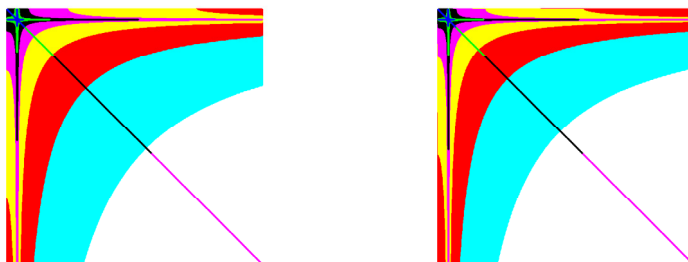
FIGURE 4.3. The size of the elements A_{2m,2n} and A_{2m+1,2n+1} for K_\omega(x, y) = e^{i\omega|x-y|} and \omega = 100 using modified Fourier basis and m, n = 0, 1, \dots, 800 .
