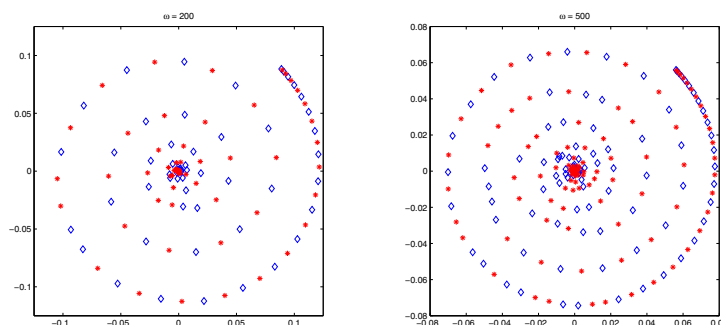
FIGURE 5.2. The same as Figure 5.1, except for \omega = 200 (on the left) and \omega = 500 . the spectrum for \omega = 100 (as obtained with the finite section method, using modified Fourier basis with r = 127 and s = 800 ) in Figure 5.1. Similar information is presented in Figure 5.2 for \omega = 200 and \omega = 500 . Evidently, the eigenvalues lie on a spiral. What is this spiral? How does it vary with \omega ?
