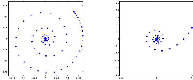
FIGURE 1.1. The spectra for g(x, y) = (x-y)^2 and g(x, y) = (x-y)^4 with \omega = 100 .
