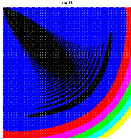
FIGURE 4.2. The size of the elements of A_{m,n} in the Legendre expansion for the Fox-Li operator with \omega = 100 .
