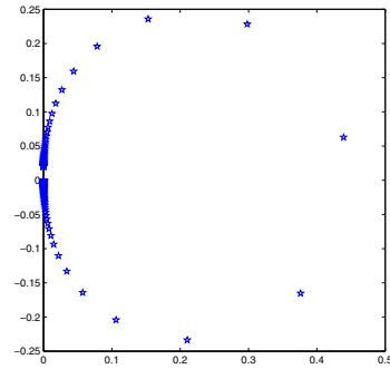
FIGURE 1.2. The spectrum for g(x, y) = |x - y| with \omega = 100 .
