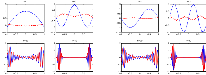
FIGURE 5.3. Real and imaginary parts of the eigenfunctions corresponding to the first, second, twentieth and fortieth ‘even’ and ‘odd’ eigenvalues, respectively, for \omega = 100 .
