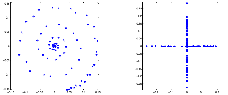
FIGURE 1.3. The spectra for g(x, y) = \cos[(1/2)\pi(x-y)] and g(x, y) = \cos[\pi(x-y)] with \omega = 100 .
