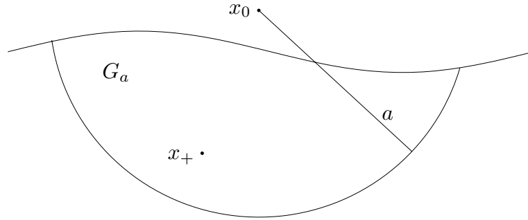
FIGURE 5. The domain G_a and points x_0, x_+ .
