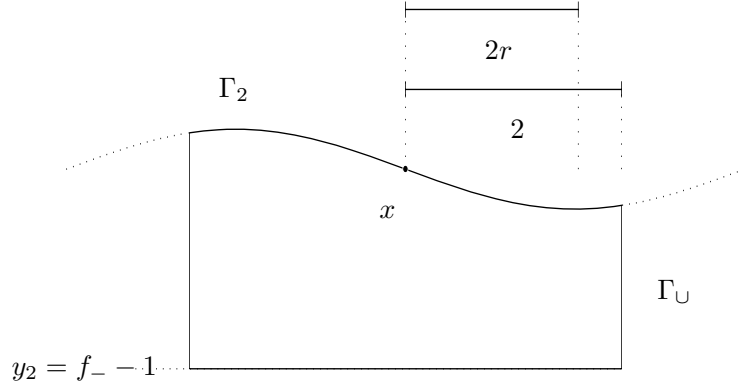
FIGURE 2. The point x , the surfaces \Gamma_2 and \Gamma_U .
