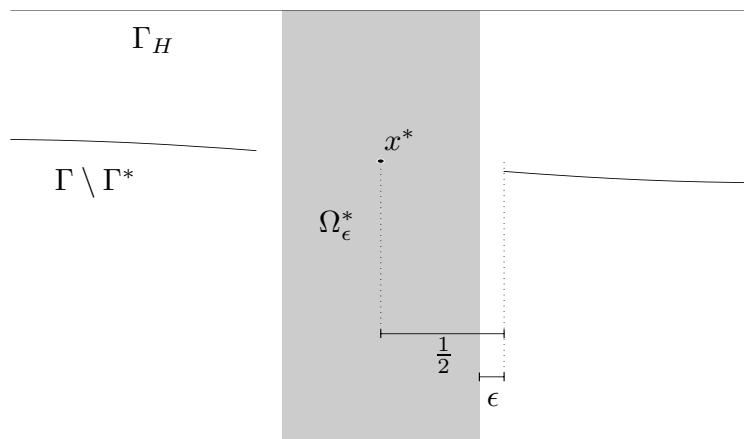
FIGURE 4. The point x^* , the surface \Gamma \setminus \Gamma^* and the domain \Omega_\epsilon^* .
