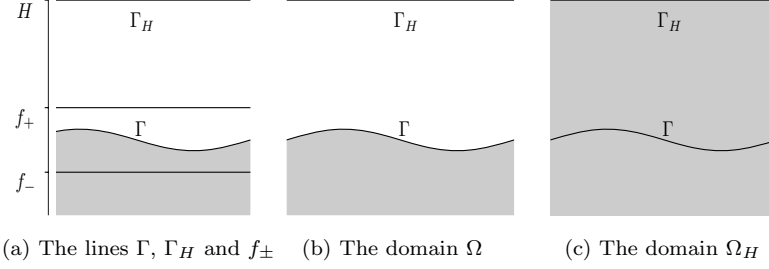
FIGURE 1. The domain for the boundary value problem.
