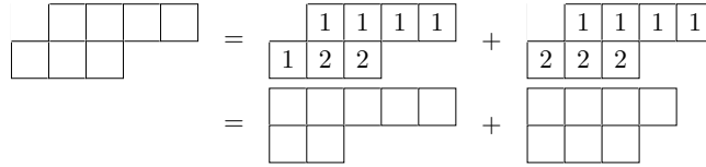
FIGURE 3. The Littlewood-Richardson rule showing S_{(5,3)/(1,0)} = S_{(5,2)} + S_{(4,3)} .
