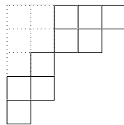
FIGURE 2. Skew diagram representing (5, 4, 2, 2, 1)/(2, 2, 1, 0, 0) .
