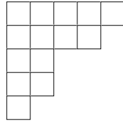
FIGURE 1. Young diagram representing (5, 4, 2, 2, 1) .
