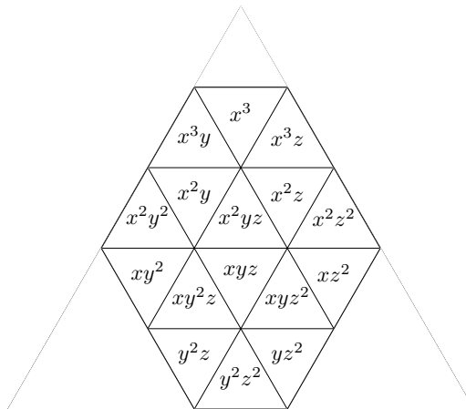
FIGURE 8. Truncating equilateral triangle.
