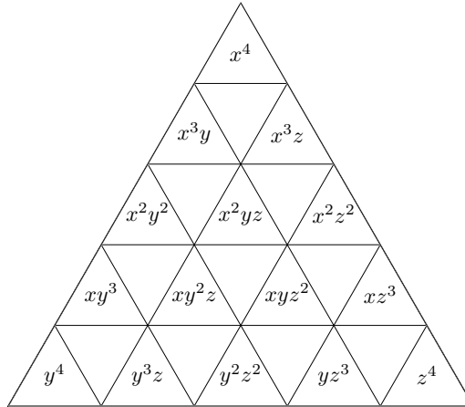
FIGURE 6. Monomials in B_4 .
