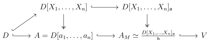
FIGURE 1. Rings involved in the proof of Proposition 4.3.
