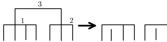
Figure 2: The ordered partition (\{1, 3, 4\}, \{5, 7\}, \{2, 6\}) is mapped to the noncrossing partition \{\{1\}, \{2, 6\}, \{3, 4\}, \{5\}, \{7\}\} .
