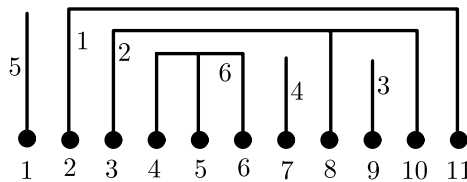
Figure 1: A monotone partition (\{2, 11\}, \{3, 8, 10\}, \{9\}, \{7\}, \{1\}, \{4, 5, 6\}) . Each block is labeled by a number to clarify the order on the blocks.
