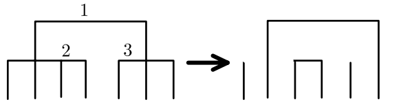
Figure 3: The ordered partition (\{2, 6\}, \{1, 3, 4\}, \{5, 7\}) is mapped to the noncrossing partition \{\{1\}, \{2, 6\}, \{3, 4\}, \{5\}, \{7\}\} .
