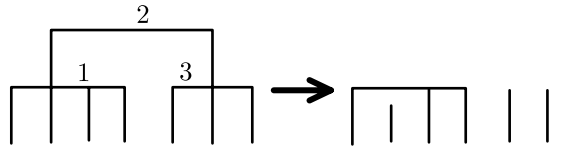
Figure 4: The ordered partition (\{1, 3, 4\}, \{2, 6\}, \{5, 7\}) is mapped to the noncrossing partition \{\{1, 3, 4\}, \{2\}, \{5\}, \{6\}, \{7\}\} .
