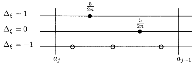
FIG. 1. Point masses for the reduced data NPMLE of F .
