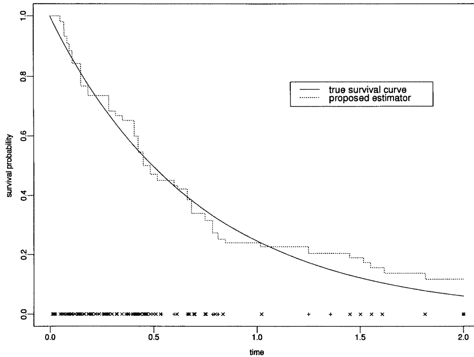
FIG. 3. The estimator \hat{S}_T based on k = 60 grid points over the interval [0, 2] . See the caption for Figure 2.
