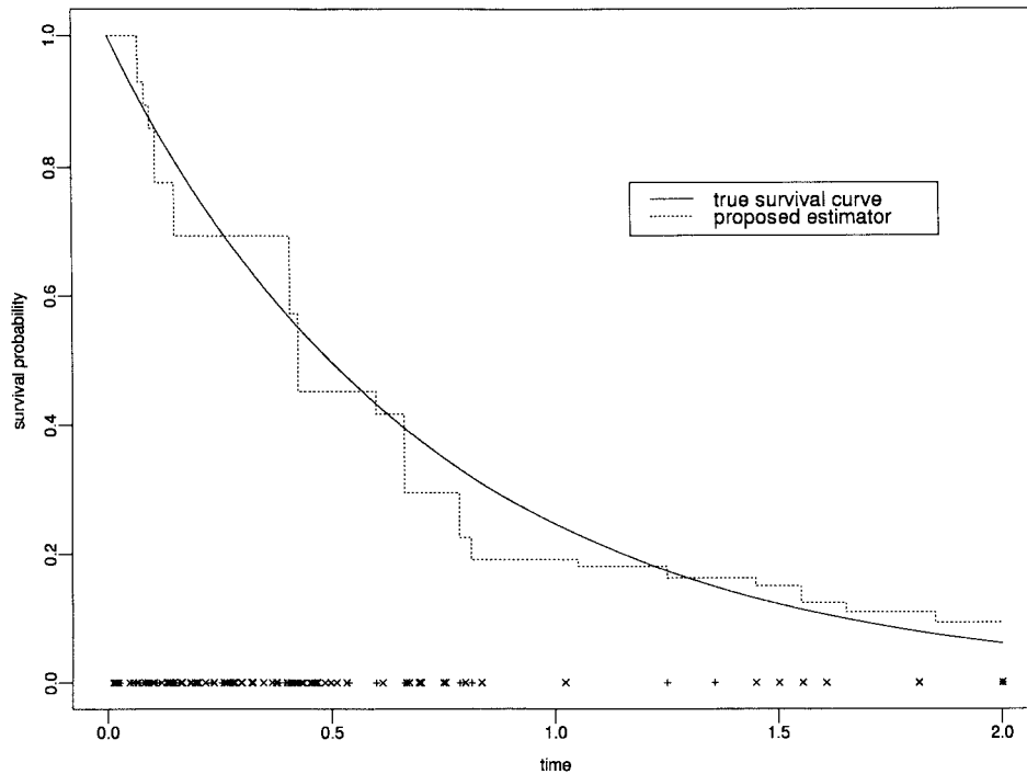
FIG. 4. The estimator \hat{S}_T based on k = 20 grid points over the interval [0, 2] . Same data as in Figure 2.
