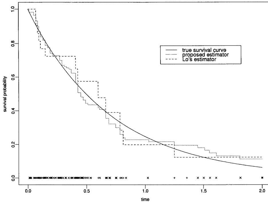
FIG. 2. The estimator \hat{S}_T compared with Lo's estimator for simulated data. The data were generated using the MCAR model in Table 1 with 30% censoring and \pi = 0.2 . The partition uses k = 100 equispaced points over the interval [0, 2] . Sample size n = 100 . The data points with missing failure indicators are represented by \times and the remaining data points by + .
