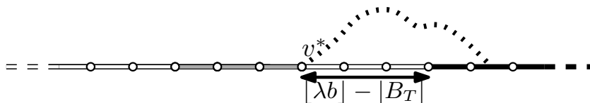
Figure 14: The crossing event C_\lambda^1 .
