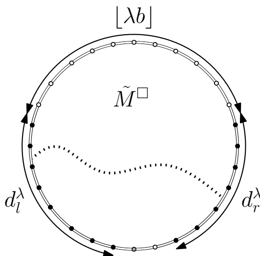
Figure 22: The event C_\lambda^2 .
