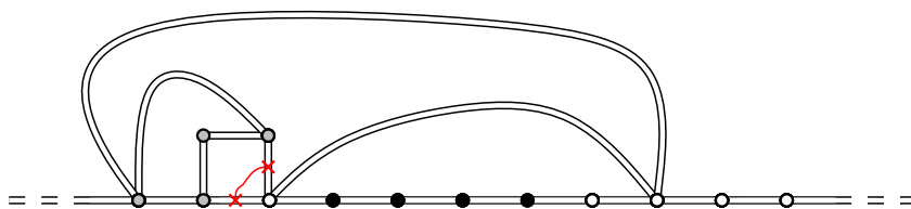
Figure 9: The situation when the algorithm ends.
