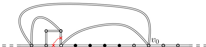
Figure 10: The situation when the finite black segment on the boundary is swallowed.
