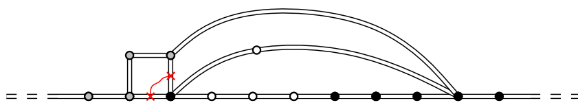
Figure 25: No black crossing occurs.
