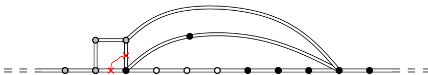
Figure 24: A black crossing occurs.
