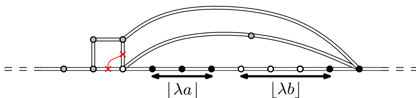
Figure 21: The situation when |B_T| > \lfloor \lambda b \rfloor .
