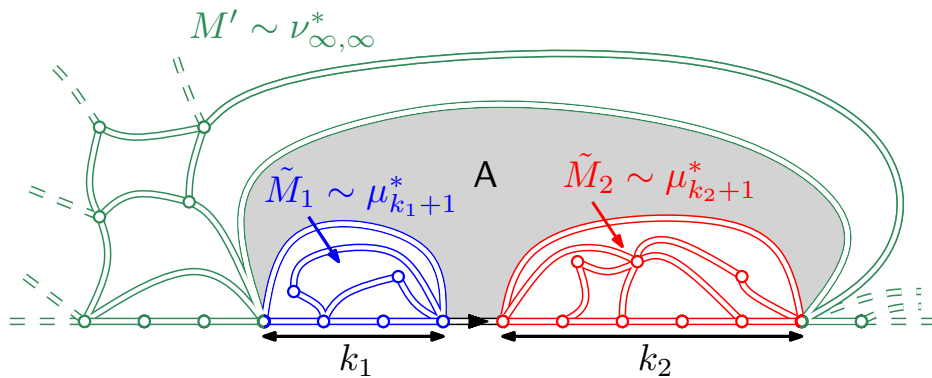
Figure 3: The spatial Markov property.
