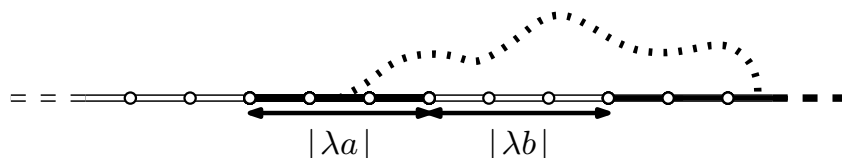
Figure 11: The boundary condition and the crossing event C^*(\lambda a, \lambda b) .
