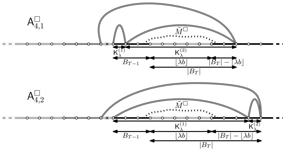
Figure 16: The likely subcases on the event A_4^{\square} .
