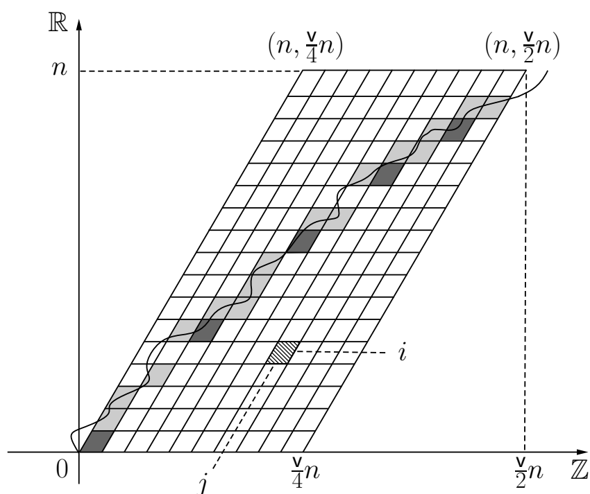
Figure 4: Construction of the trajectories of blocks, \mathcal{R} and \mathcal{T} , from a deterministic trajectory (k, Y_k)_{0 \leq k \leq n} satisfying Y_0 = 0 and Y_n \geq \frac{v}{2}n . The trajectory \mathcal{R} is marked by the shaded boxes, and the trajectory \mathcal{T} \subset \mathcal{R} by the darker boxes. A box C(i, j) is represented by the hatched region.
