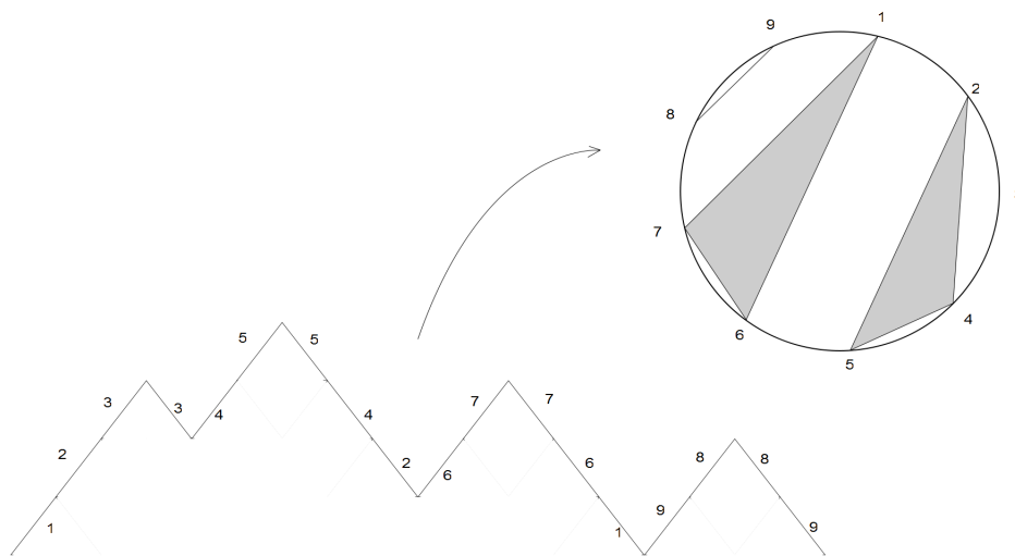
Figure 2: An example for the bijection \Phi .
