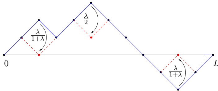
Figure 2: Three possible transitions, with the corresponding rates, for the model without the wall.
