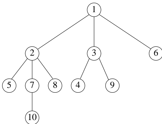
Figure 1: A recursive tree on [10] .
