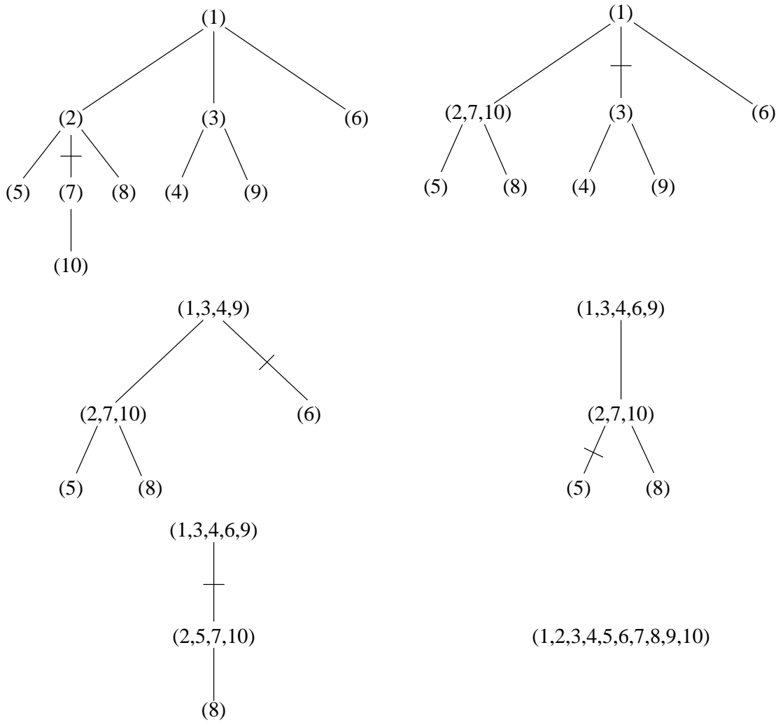
Figure 2: The cutting procedure for a random recursive tree on [10] , with the cuts indicated.
