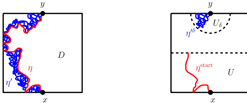
Figure 10: Left. For the imaginary geometry h^{\text{IG}} , the angle \frac{\pi}{2} flow line \eta is a.s. the right boundary of the counterflow line \eta' (Lemma B.2). Right. The initial segments \eta^{\text{start}} and \eta'^\delta are a.s. determined by h|_U and h|_{U_\delta} , respectively.
