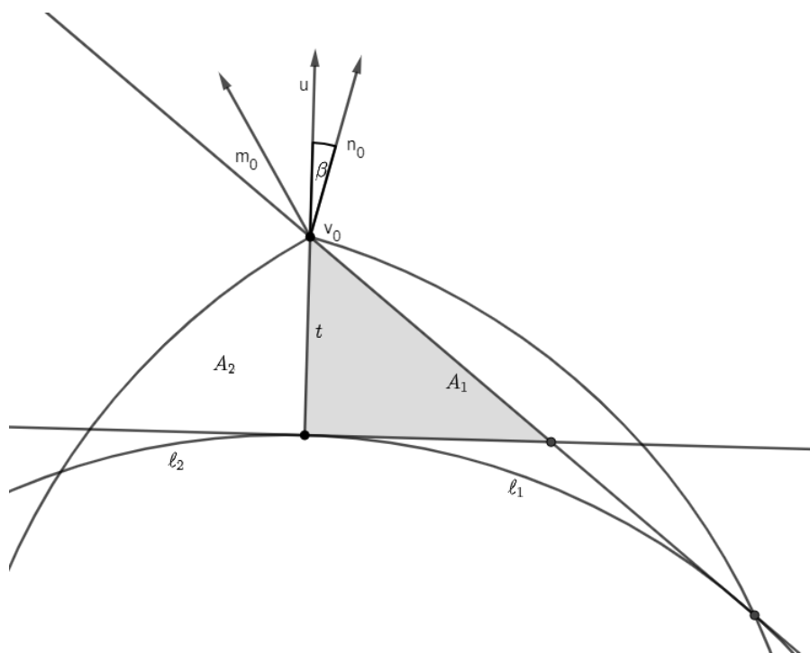
Figure 2: Disc-cap D(\beta, t)
