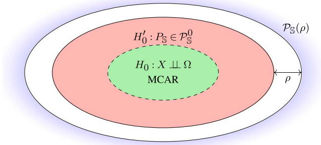
FIG. 1. Illustration of our minimax testing framework.
