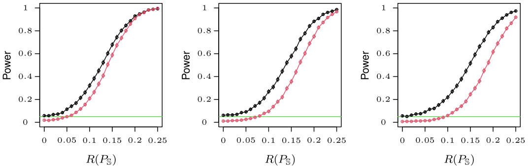
FIG. 3. Power curves for our Monte Carlo test (black) and Fuchs’s test (red). Error bars show three standard errors. Here, \mathbb{S} = \{\{1, 2\}, \{2, 3\}, \{1, 3\}\} with \mathcal{X} = [r] \times [2]^2 and r = 2 (left), r = 4 (middle) and r = 6 (right).
