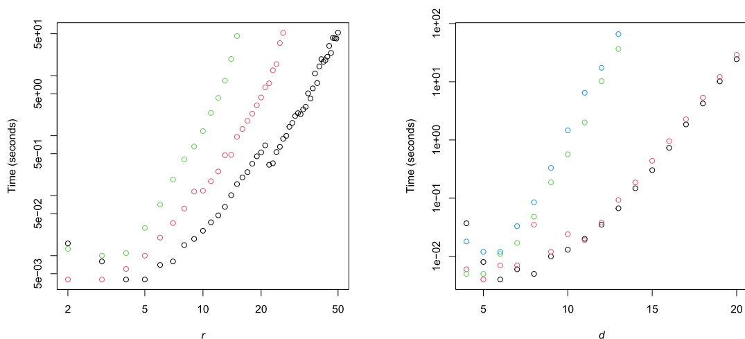
FIG. 5. Time taken to compute R(\cdot) in various settings. In the left-hand plot the d = 3, 4, 5 examples are represented by the black, red and green points, respectively. In the right-hand plot the r = 2 results are shown in black and red for m = 2, 3 , respectively, and the r = 3 results are shown in green and blue for m = 2, 3 , respectively.
