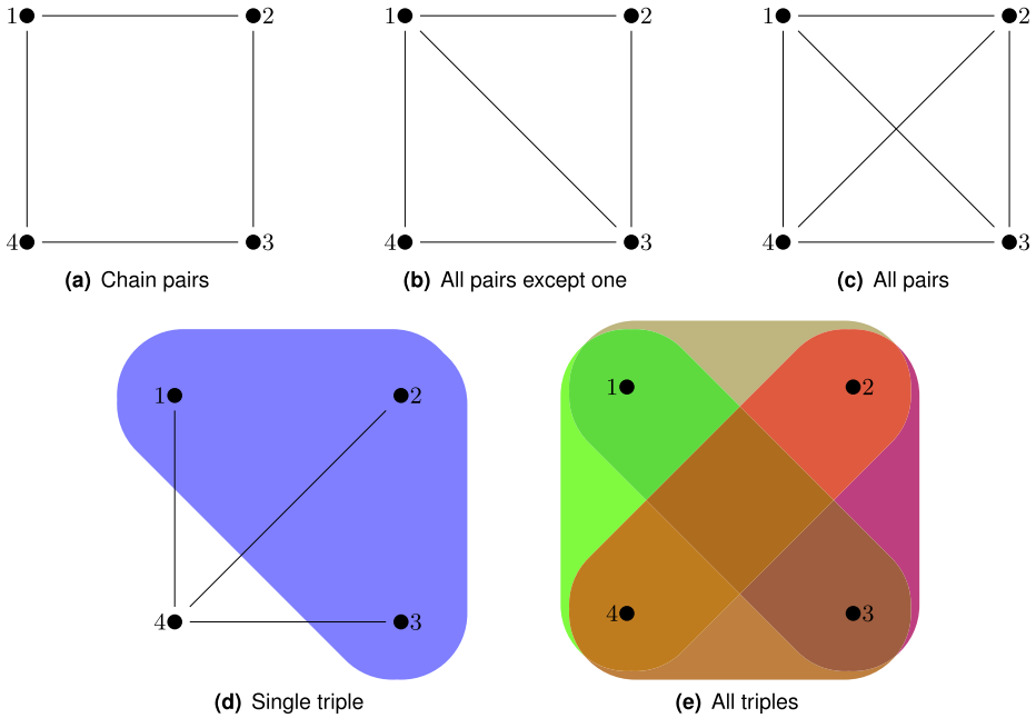
FIG. 2. Irreducible observation patterns \mathbb{S} with d = 4 .
