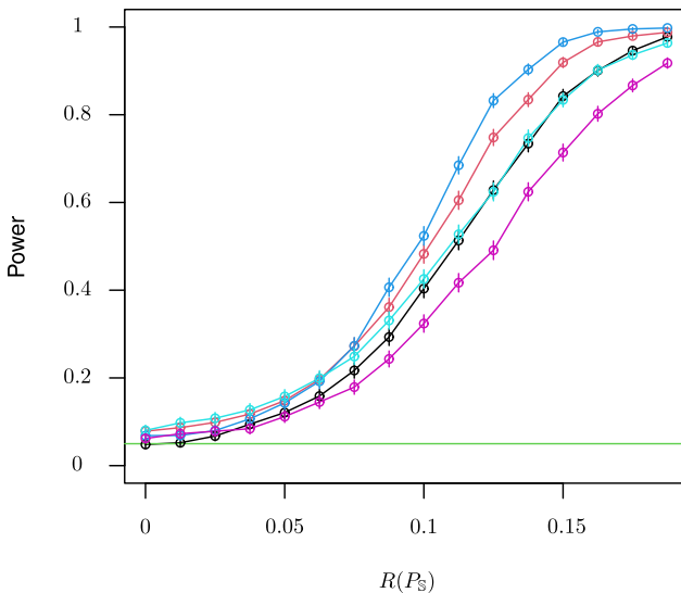
FIG. 4. Power curves for our Monte Carlo test (black) and Fuchs's test with the latter test being applied with an additional n_{\{1,2,3,4,5\}} = 25 (magenta), 50 (cyan), 100 (red) and 200 (blue) complete cases. Error bars show three standard errors. Here, \mathbb{S} = \{\{1, 2, 3, 4\}, \{1, 2, 3, 5\}, \{1, 2, 4, 5\}, \{1, 3, 4, 5\}, \{2, 3, 4, 5\}\} , with \mathcal{X} = [2]^5 .
