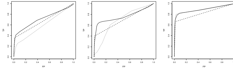
FIG 2. ROC curves ((AFGM (—), FAPO (---), FGGM (···)) for Model I (left), Model II (middle) and Model III (right).
