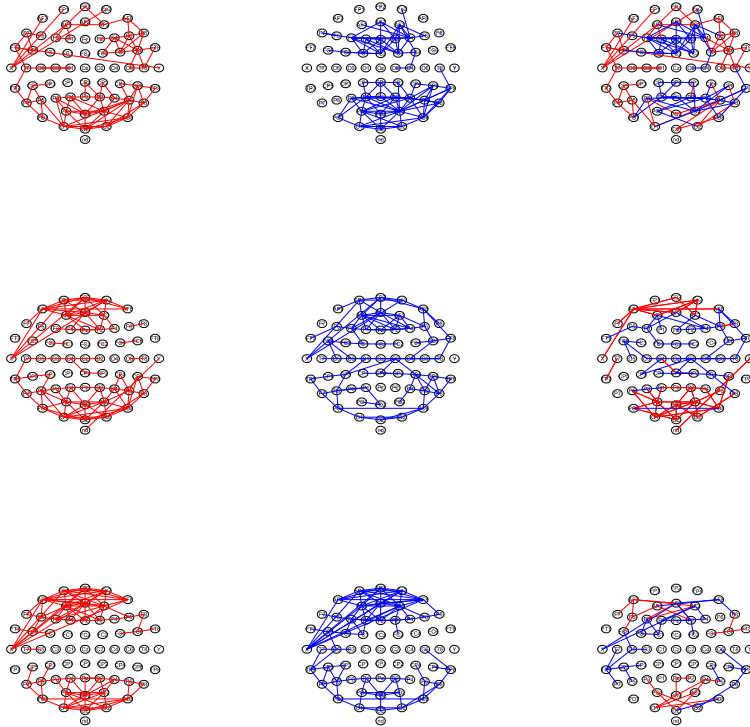
FIG 3. Estimated brain networks by AFGM (upper panels), FAPO (middle panels) and FGM (lower panels) for the alcoholic group (left), the control group (middle) and differential brain networks (right)
