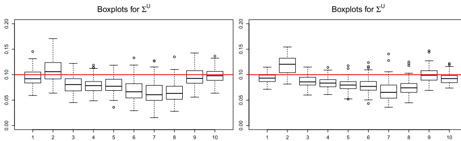
FIG 8. Simulation results for the components of (\hat{\Sigma}_{i,i}^U)_{1 \leq i \leq 10} for models \tilde{M}_1 (left) and \tilde{M}_1^{HD} (right) for the proposed procedure. The horizontal red line present the true value.
