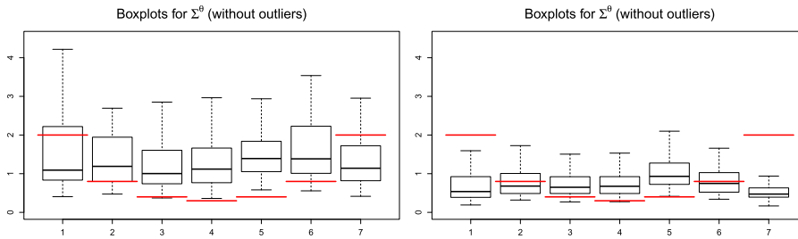
FIG 7. Simulation results for the components of (\hat{\Sigma}_{i,i}^\theta)_{1 \leq i \leq 7} for the proposed procedure for model \tilde{M}_1 (left) and \tilde{M}_1^{HD} (right). Boxplot without the outliers. True coefficient values: red horizontal lines.
