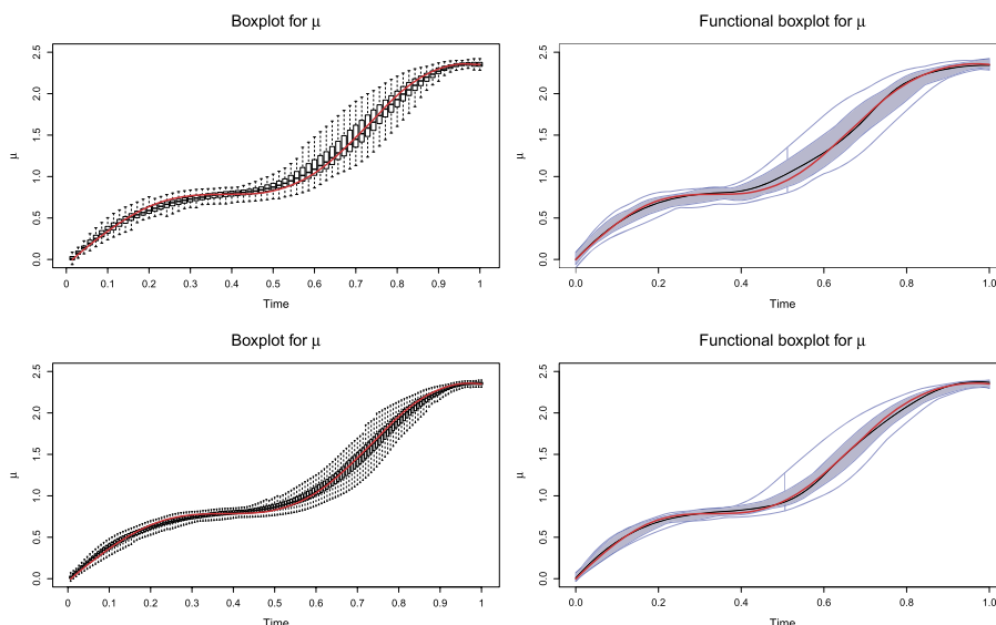
FIG 6. Comparison between \hat{\mu}_1 and \tilde{\mu}_1 for model \tilde{M}_1 ( n = 100 and T = 70 , top) and for model \tilde{M}_1^{HD} ( n = 200 and T = 150 , bottom) using the proposed method.
