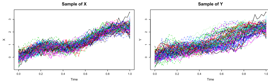
FIG 4. A sample of the warped process X (left) and the un-warped process Y (right) for M_1 .
