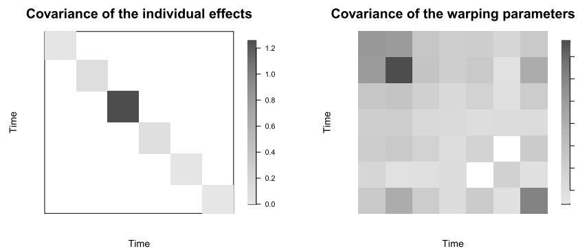
FIG 10. Estimated covariance matrices \hat{\Sigma}^U (left) and absolute value of \hat{\Sigma}^\theta (right).
