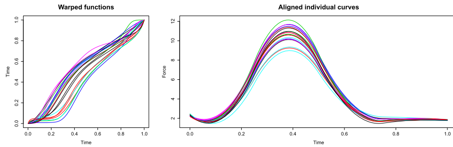
FIG 9. Estimated warping functions (left) and warped individual curves (right).
