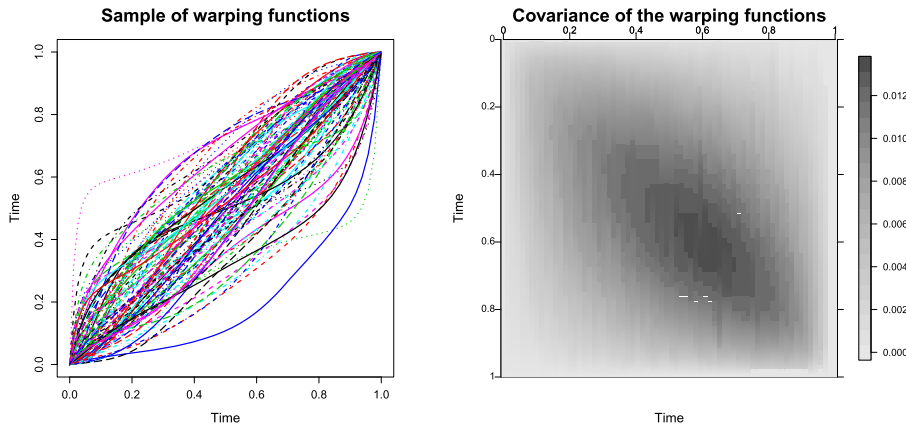
FIG 2. A sample of size 100 of warping functions (left), and the empirical covariances of these functions (right).
