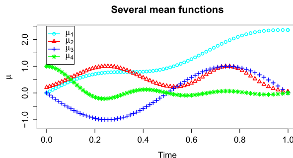
FIG 3. The mean functions \mu in the simulation study.
