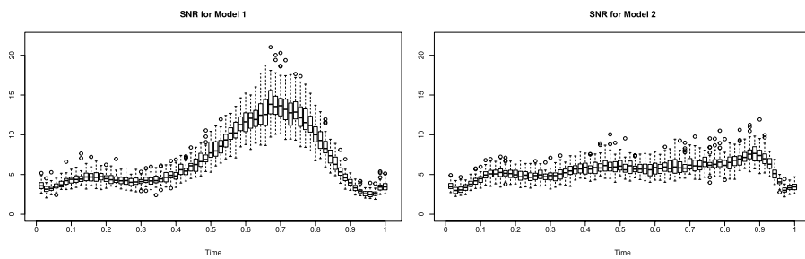
FIG 5. SNR functions for \tilde{M}_1 (left) and \tilde{M}_2 (right).
