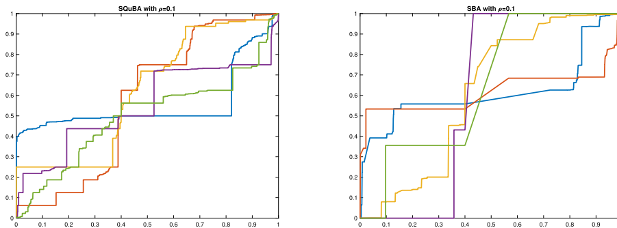
FIG 6. Five random SQA cumulative distribution function on the left and five random SBA on the right. The SQA is derived with \tau = 0.5 for an easier comparison with SBA that consider the mean. The median on the left and the mean on the right are assigned equal to 0.4. \lambda gives 0.1 mass to 0 and is uniform elsewhere.
