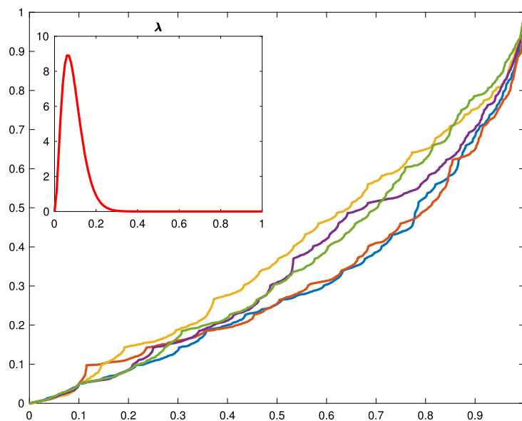
FIG 3. Five random SQA cumulative distribution function with the same \lambda that is a Beta(3, 30) . The quantile q_{1,1} is 0.1 with \tau = 0.05 .
