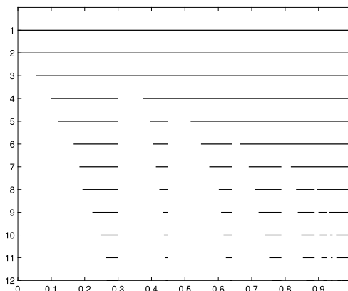
FIG 2. Graphical representation of the intervals in which q_{n,k} are simulated with \varepsilon = 10^{-3} , \tau = 0.01 . The figure shows only 12 levels, while to cover in a reasonably dense way (according to \varepsilon ) the whole intervals, 134 levels are needed.
