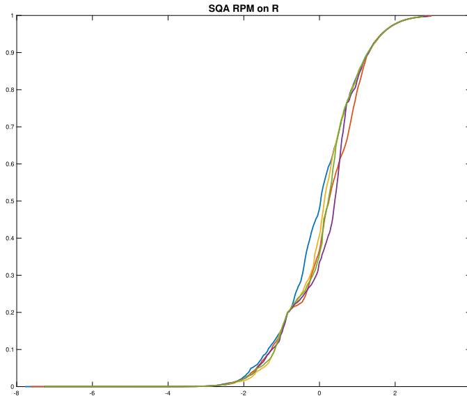
FIG 8. Five random SQA cumulative distribution function on \mathbb{R} obtained by those reported in 7(rhs) with the link function H chosen as the inverse of a standard normal.
