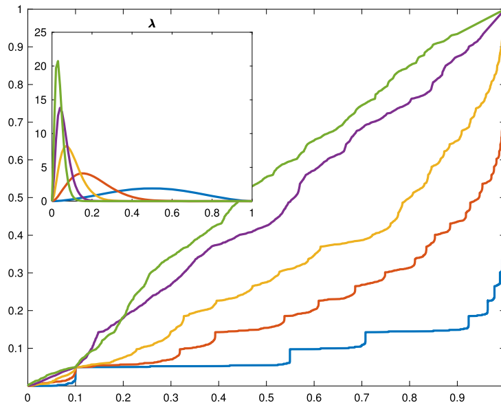
FIG 4. Five random SQA cumulative distribution function with different \lambda . The distributions \lambda are Beta(3, 3a^2) with a = 1, \dots, 5 . The quantile q_{1,1} is 0.1 with \tau = 0.05 .
