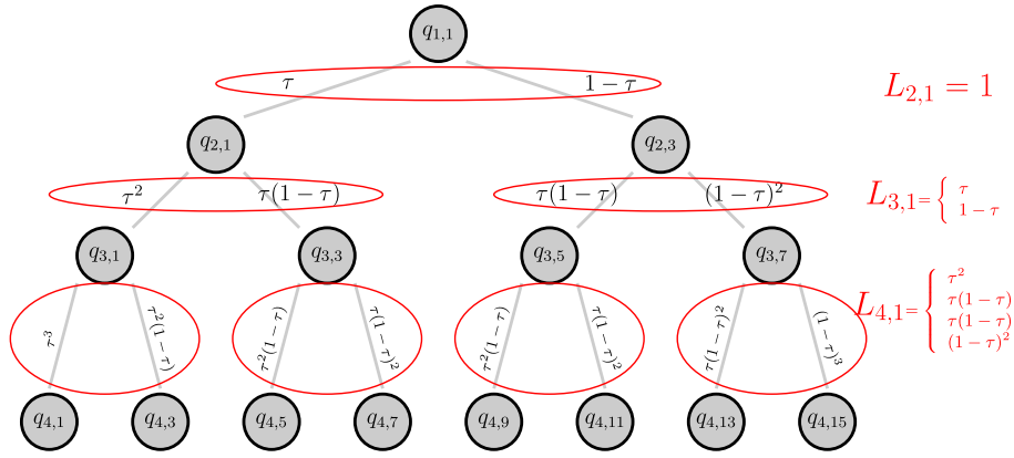
FIG 1. Set of possible total heights of the jumps L_{n,k} , when there is a single ( k = 1 ) new tie occurring at the n th step of the construction of the sequence of the quantiles, n \geq 2 . The values of L_{n,1} are given by the sum of the probabilities in each ellipse.
