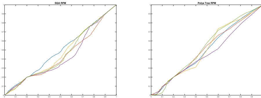
FIG 7. Five random SQA cumulative distribution functions on the left with \lambda_n changing with n . Five random Polya tree cumulative distribution function on the right. Both are derived with \tau = 0.2 and quantile 0.2. The \lambda_n in SQA are such that to satisfy conditions of Theorems 3.5, 3.6 and 3.7 while PT is simulated as in [34] using a \text{Beta}(n^2, n^2) .
