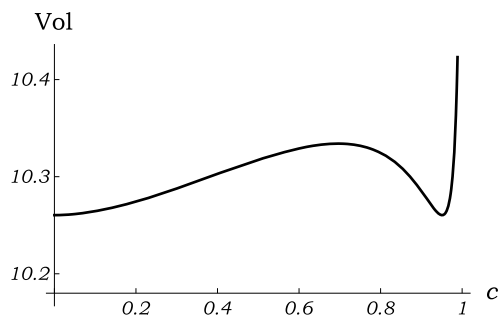
FIG 1. \text{Vol}(\gamma_{M(c)}^{-1}) for a mixing design.
