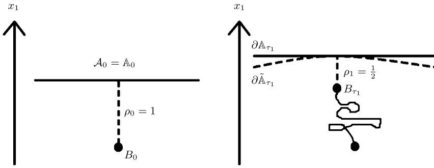
FIG. 3. The initial set \mathbb{A}_0 and the case when \rho_1 = 1/2 .
