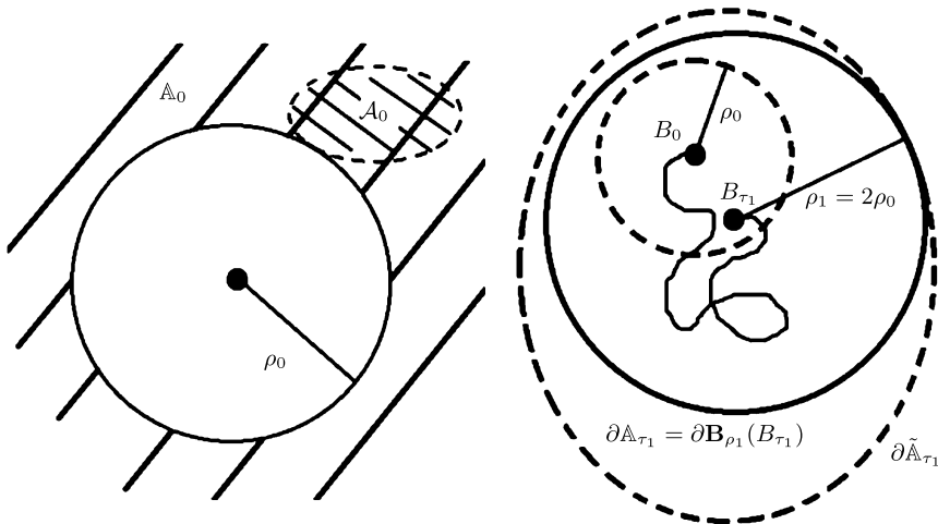
FIG. 1. The initial set \mathbb{A}_0 and the case when \rho_1 = 2\rho_0 .
