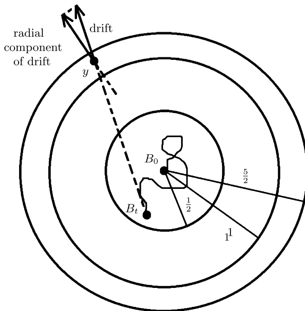
FIG. 2. The projection of the drift onto the radial direction.
