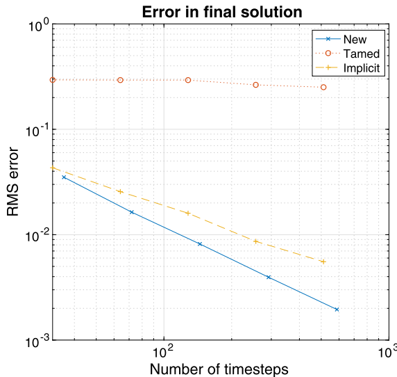
FIG. 6. Numerical results for FENE model in finite time interval.
