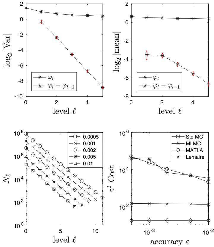
FIG. 3. Adaptive MLMC for invariant distribution.
