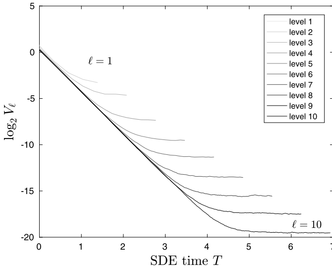
FIG. 2. Variance of corrections on each level \ell .
