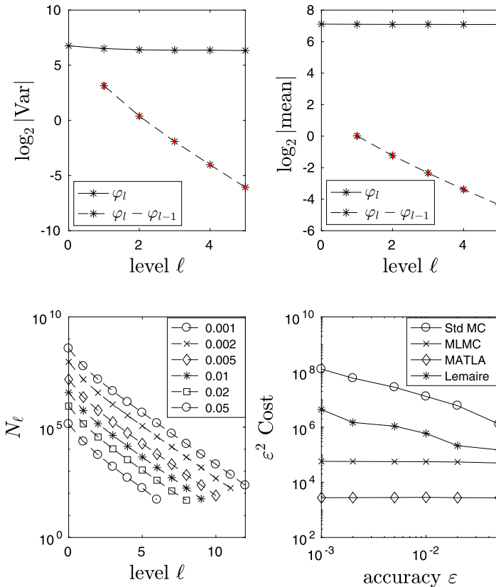
FIG. 5. Adaptive MLMC for invariant distribution (double well).
