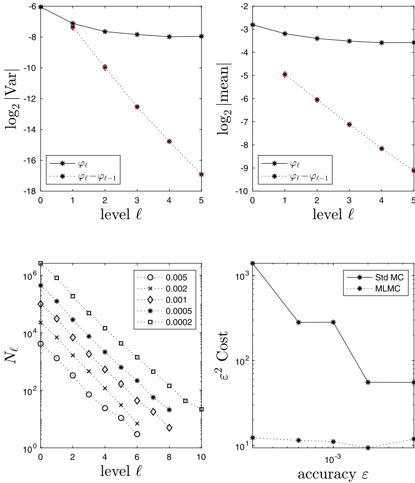
FIG. 7. Adaptive MLMC for invariant distribution (FENE).
