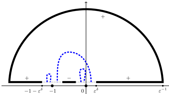
FIG. 9. Signs of \text{Im } \mathbf{S}'(z) along the curves described in Lemma 5.2. Blue dashed curves represent a possible part of the boundary of the set \mathcal{U} inside \mathcal{D} ; see Lemma 5.4 below.
