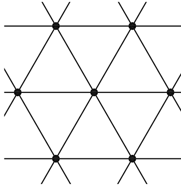
Fig. 2. Triangular lattice.
