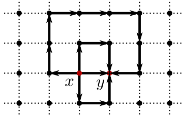
Fig. 1. Independent paths.
