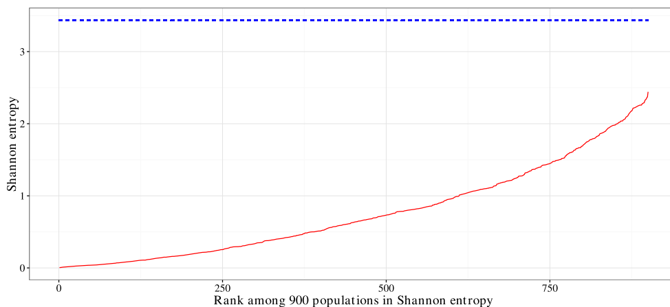
FIG. 1. The empirical Shannon entropy in the microbial distribution across 900 samples of the vaginal microbiome (Ravel et al. [59]), which are ranked according to the level of diversity. The dashed blue line shows the Shannon entropy of the Uniform distribution for the same number of species.
