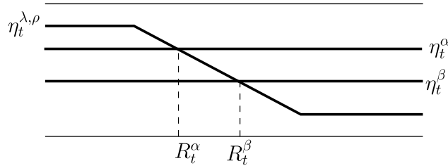
FIG 9.3. Macroscopic schema of (9.12)-(9.13)
