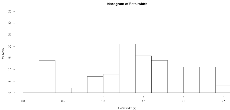
Figure 1 Histogram of Petal width.
