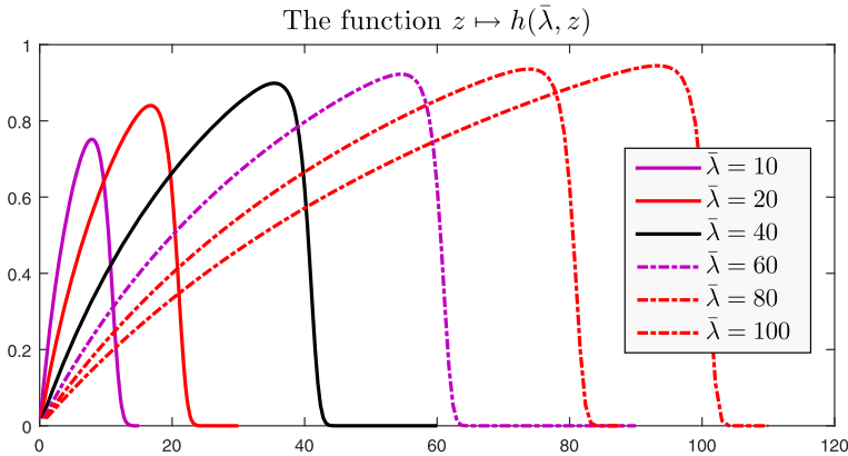
FIG. 2. For different values \bar{\lambda} \in \{10, 20, 40, 60, 80, 100\} , we plot the function z \mapsto h(\bar{\lambda}, z) .
