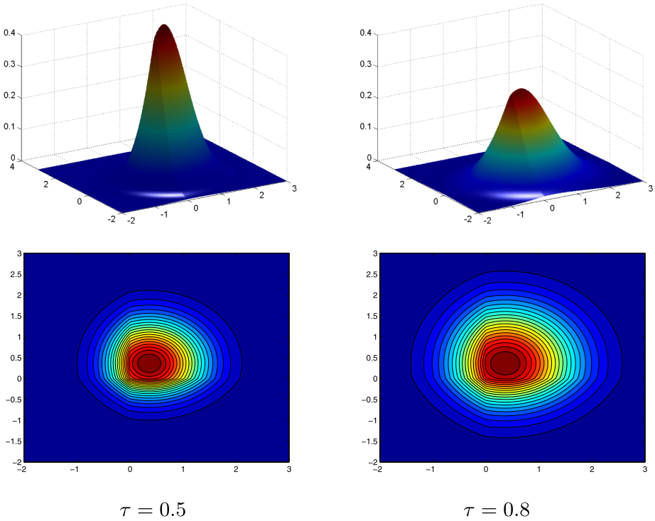
FIG. 1. Top: the plots of the pseudo-posterior \hat{\pi}_n with the Laplace prior for the temperature \tau = 0.5 (left) and \tau = 0.8 (right). One can observe that decreasing the value of \tau strengthens the peakedness of the density. Bottom: the level curves of the pseudo-posterior \hat{\pi}_n with the Laplace prior for the temperature \tau = 0.5 (left) and \tau = 0.8 (right). One clearly observes the nondifferentiability of the density along the axes \beta_1 and \beta_2 (caused by the nondifferentiability of the \ell_1 -norm).
