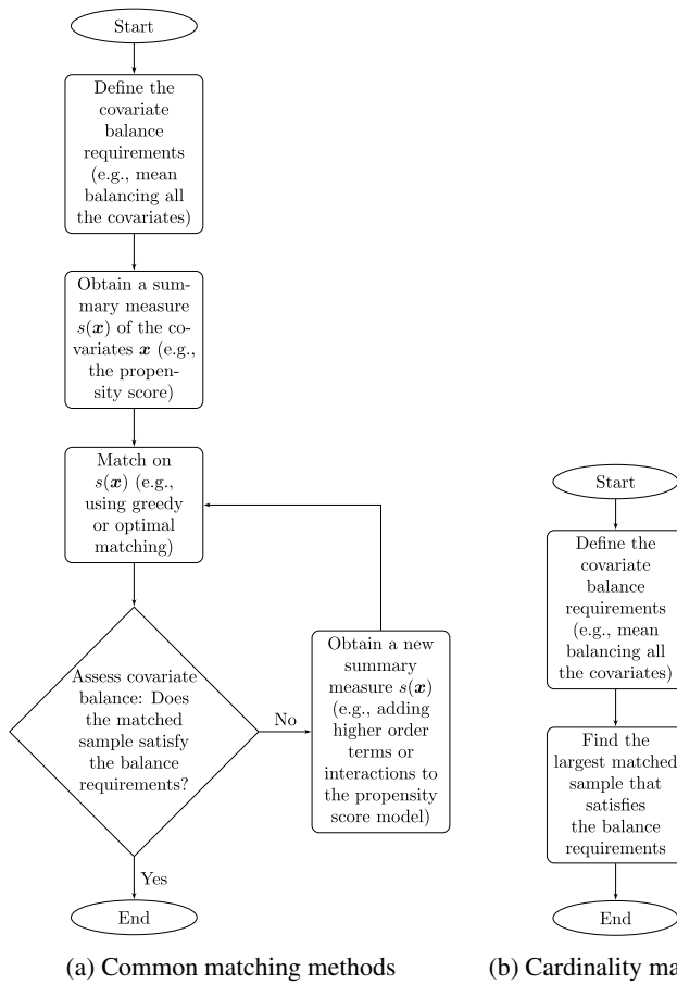
FIG. 1. Flowcharts of common matching methods and cardinality matching.
