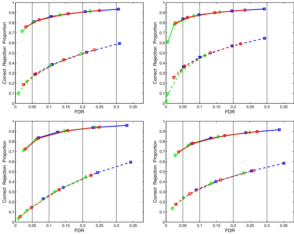
FIG. 1. Performance comparison of B - H procedures based on three calibration methods in \text{Sim}_1 with (n_1, n_2) = (50, 30) and m = 1000 . The first and second rows show the results when the components of noise vectors \boldsymbol{\varepsilon}_1 and \boldsymbol{\varepsilon}_2 follow t -distributions and exponential distributions, respectively; left and right panels show the results for homogeneous and heteroscedastic cases, respectively; horizontal and vertical axes depict empirical false discovery rate and empirical correct rejection proportion, respectively; and the prescribed levels \alpha = 0.05, 0.1, 0.2 and 0.3 are indicated by unbroken horizontal black lines. In each panel, dashed lines and unbroken lines represent the results for the discrepancy parameter c = 1 and 1.5 , respectively, and different colors express different methods employed to calculate p -values in the B - H procedure, where blue line, green line and red line correspond to the procedures based on normal, conventional and regularized bootstrap calibrations, respectively.
