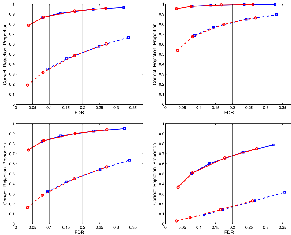
FIG. 2. Performance comparison of B - H procedures based on two different calibration methods in \text{Sim}_2 with (n_1, n_2) = (50, 30) and m = 1000 . The first and second rows show the results when the components of noise vectors \mathbf{e}_1 and \mathbf{e}_2 follow the distributions specified in cases 1 and 2 of Table 2, respectively; left and right panels show the results for the cases of identical distributions and non-identical distributions, respectively; horizontal and vertical axes depict empirical false discovery rate and empirical correct rejection proportion, respectively; and the prescribed levels \alpha = 0.05, 0.1, 0.2 and 0.3 are indicated by unbroken horizontal black lines. In each panel, dashed lines and unbroken lines represent the results for the discrepancy parameter c = 1 and 1.5 , respectively, and different colors express different methods employed to calculate p -values in the B - H procedure, where blue line and red line correspond to the procedures based on normal and bootstrap calibrations, respectively.
