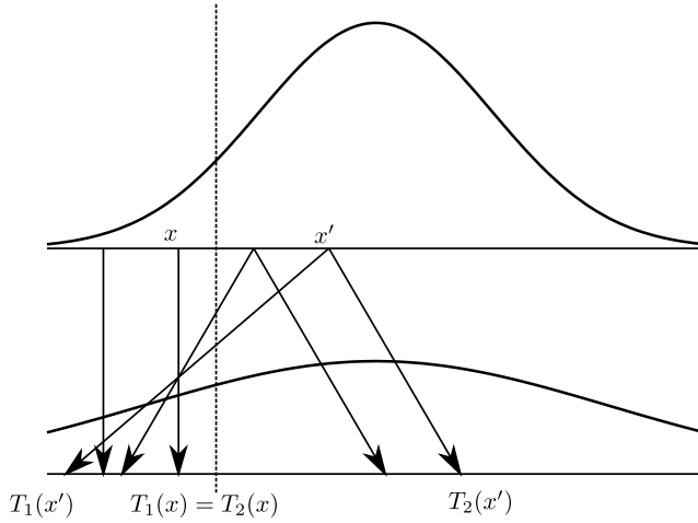
FIG. 2. Scheme of the left-curtain \pi_{1c} coupling between two Gaussian measures.
