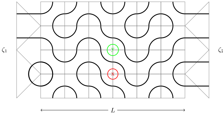
FIG. 6. A particular configuration of the dense loop model showing a path passing between two vertically adjacent points x and y .
