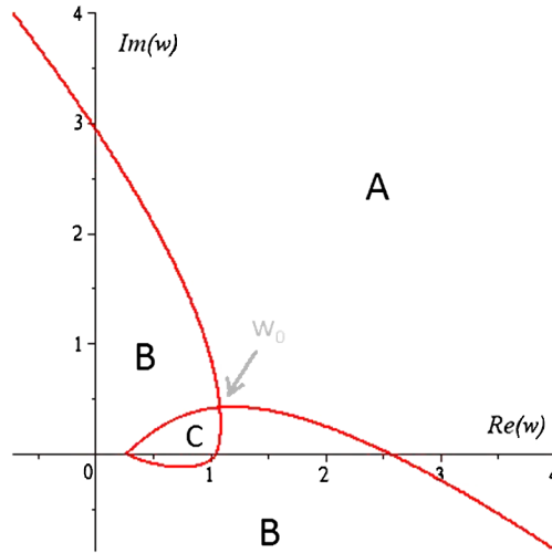
FIG. 7. Sketch of the level lines \text{Re}(yw - \mathcal{F}(w; 0)) = \text{Re}(yw_0 - \mathcal{F}(w_0; 0)) for y = 1 - i .
