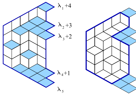
FIG. 1. Lozenge tiling of the domain encoded by signature \lambda (left panel) and of corresponding polygonal domain (right panel).
