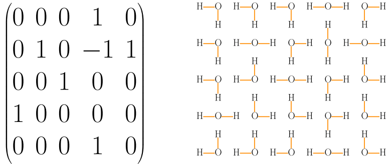
FIG. 4. An alternating sign matrix of size 5 and the corresponding configuration of the six-vertex model (square ice) with domain wall boundary condition. 1s in ASM correspond to horizontal molecules H-O-H and -1s to the vertical ones.
