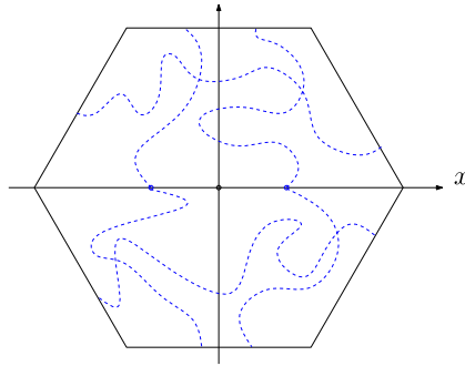
FIG. 7. The events \mathcal{C}^{U_n}, \mathcal{C}^{L_n}, \mathcal{T}_+^n, \mathcal{T}_-^n .
