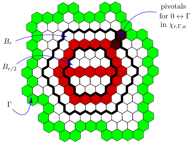
FIG. 4. The boundary paths delimiting B_2 and B_4 are black, and the circuit \Gamma is light green. The darker (red and brown) hexagons are the open hexagons of \chi_{4,\Gamma,2} : the red hexagonal circuit is set in such a way that its distance from \Gamma is a = 2 , and the brown path is chosen in some arbitrary but fixed way so that it realizes this distance a . Note that this brown path is the set of pivots for 0 \leftrightarrow \Gamma .
