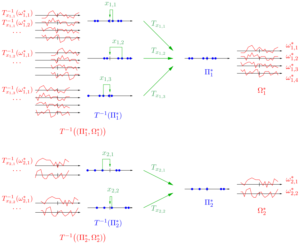
FIG. 3. A schematic picture of the effect of Liggett’s extra head time shift T on (\Pi_{\mu_r}, \omega) . [For simplicity, the figure pretends that \Pi is a measurable function of \omega , instead of (\omega, \Theta) .] Different Palm point process realizations \Pi_1^* and \Pi_2^* may arise from a different “amount” of Palm dynamical percolation realizations \Omega_1^* = \{\omega_{1,i}^* : i \in I_1\} and \Omega_2^* = \{\omega_{2,i}^* : i \in I_2\} (a ratio 4 : 2 on the right-side of the picture), and the preimages T^{-1}(\Pi_1^*) and T^{-1}(\Pi_2^*) might also have different sizes (which gives the reweighting of the Palm measure compared to the ordinary measure, a ratio 3 : 2 in the middle of the picture). The product of these ratios is the same as the ratio for the preimages T^{-1}((\Pi_1^*, \Omega_1^*)) and T^{-1}((\Pi_2^*, \Omega_2^*)) .
