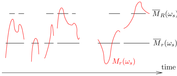
FIG. 1. Schematic pictures of the approximate local time densities for \bar{\mu}_r and \mu_r .
