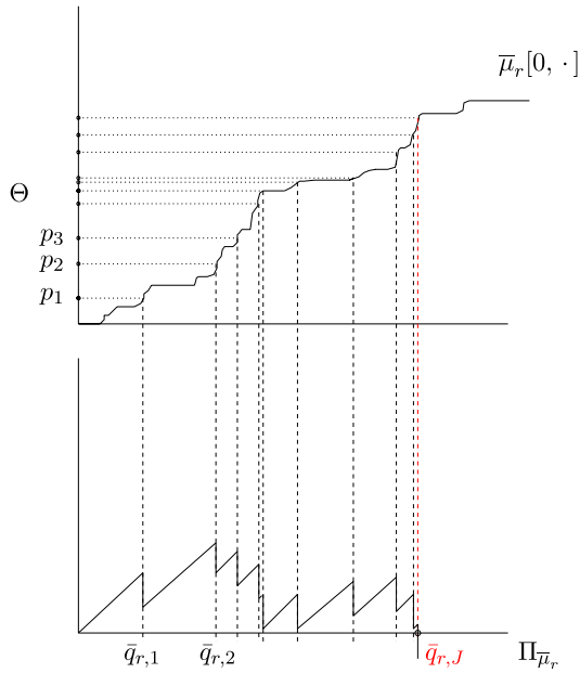
FIG. 2. Depicting Liggett's extra head construction.
