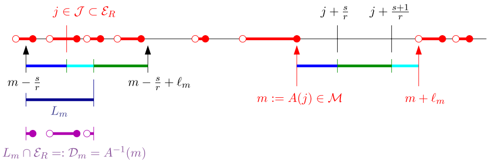
FIG. 5. The domain of attraction \mathcal{D}_m appearing in the definition of \mathbb{P}'' , and the map A: \mathcal{J} \rightarrow \mathcal{M} appearing in the proof of \mathbb{P}'' = \mathbb{P} (Lemma 4.15).
