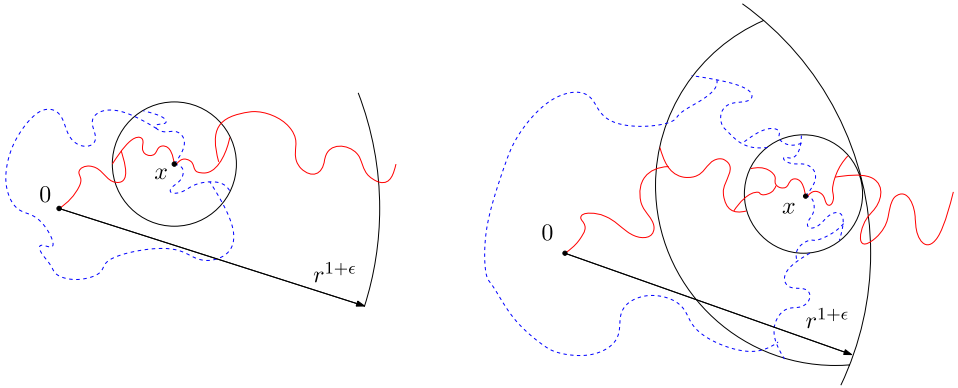
FIG. 6. Conditioned on 0 \leftrightarrow r^{1+2\epsilon} , one 4-arm event (first picture) or one 4-arm and one 3-arm events (second picture) are roughly equivalent to x being pivotal for 0 \leftrightarrow r^{1+\epsilon} .
