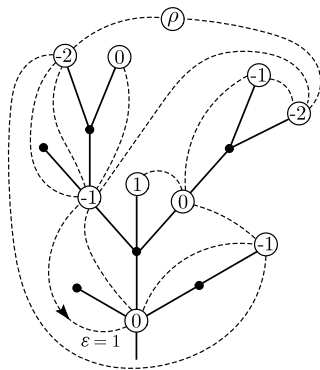
FIG. 2. An illustration of the BDG bijection. The edges in the mobile are solid and the edges in the planar map are dashed.
