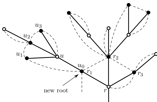
FIG. 3. A diagram describing the bijection from \Gamma_n to itself which sends white vertices to vertices of degree 1 and black vertices of degree k to vertices of degree k + 1 .
