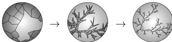
FIG. 1. The convergence in Theorem 1.1. A face of large degree (light gray) appears as the planar map gets larger and the boundary of that face collapses into a tree.
