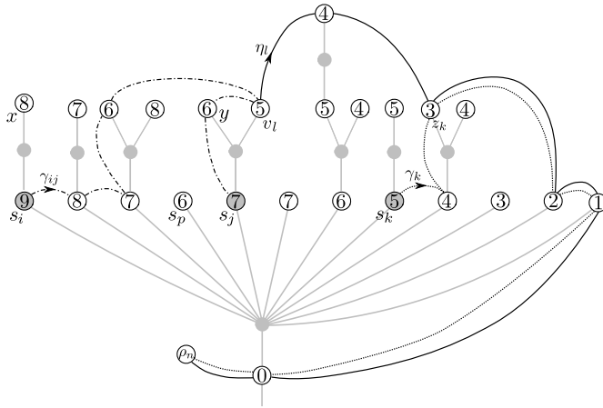
FIG. 6. Illustration of the setup in part (3) of the proof with \ell_n(s_k) = 5 , \lambda_2 = 5 and \lambda_3 = 4 . A planar mobile is shown with the edges and the black vertices colored light gray. The geodesic \gamma_{ij} is dotted and dashed, \eta_l is solid and \gamma_k is dotted. Since \eta_l and \gamma_k are successor geodesics, they intersect at the vertex z_k with label \lambda_3 - 1 = 3 .
