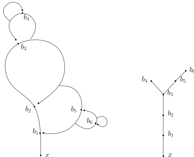
Fig. 2. Example of a collection of cycles and the corresponding tree \mathbf{T}_x .
