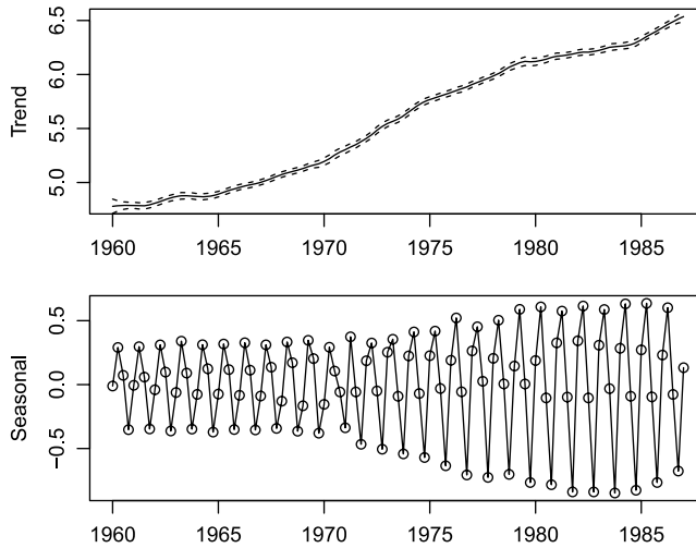
Figure 5 UK gas consumption: trend and seasonal component, with 95% credible intervals using the Student-t-Beta(4, 1, 1, \frac{1}{\beta} = 10,000 ).
