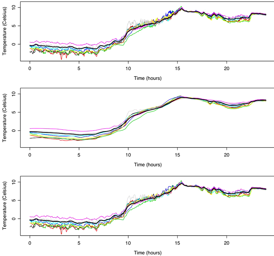
Figure 7 Effect of variance estimation on reconstruction. Top: wavethresh smoothing using default settings; middle: wavethresh smoothing with modified settings; bottom: reconstruction after applying the hierarchical model, with the error variance fixed beforehand as the variance of the coefficients at level 3 and higher.
