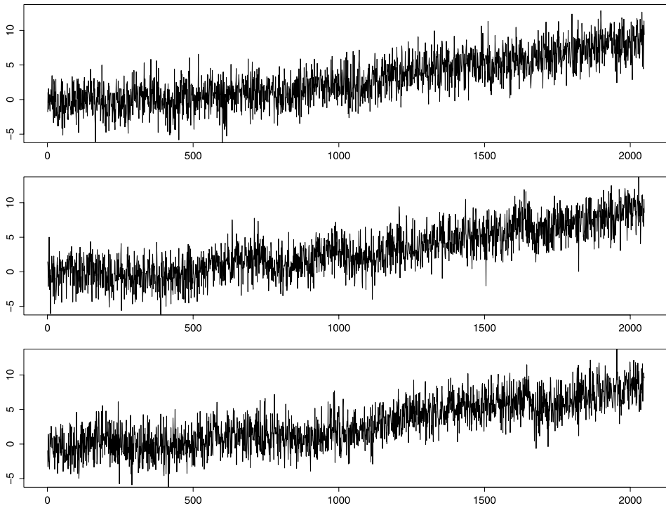
Figure 2 Three time series obtained by applying the inverse discrete wavelet transform to sets of simulated wavelet coefficients.
