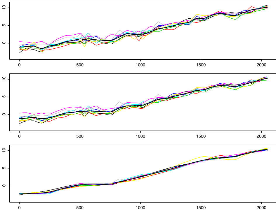
Figure 3 Reconstructed time series obtained by applying inverse discrete wavelet transform to, from top to bottom, the true wavelet coefficients, the coefficients estimated with the median rule via empirical Bayes, and the coefficients after thresholding with wavethresh using default settings. Narrow lines: the eight station-specific smooth signals, thick line: the underlying mean signal (in the bottom panel, the pointwise mean of the station-specific smooth signals).
