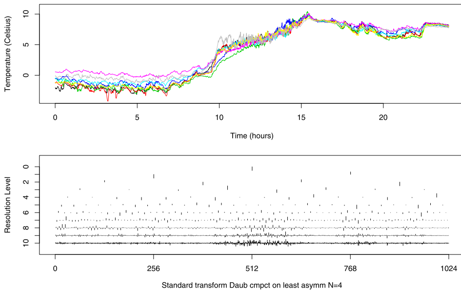
Figure 5 Example series from the SensorScope data. Top: eight time series consisting of SensorScope air temperature data taken over 24 hours. Bottom: wavelet decomposition of one of the series.
