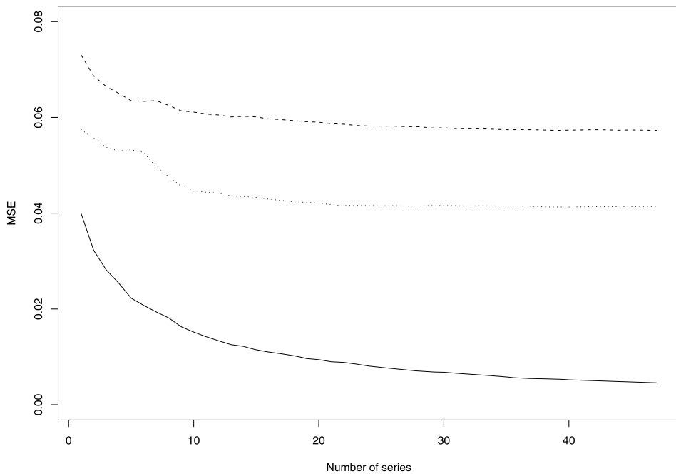
Figure 4 Mean square errors (MSE) for different estimation methods, based on 50 replicates with different numbers of stations. The lines show: MSE of the posterior median estimates (solid) and wavethresh estimates (dashes) of the grand mean coefficients \zeta_{jk} , with the wavethresh estimates simply the mean of the thresholded coefficients; and MSE of the posterior median estimates of the signal-specific coefficients v_{jk}^{(s)} (dots). wavethresh estimates for these have an MSE of about 0.14, which does not decrease with the number of stations.
