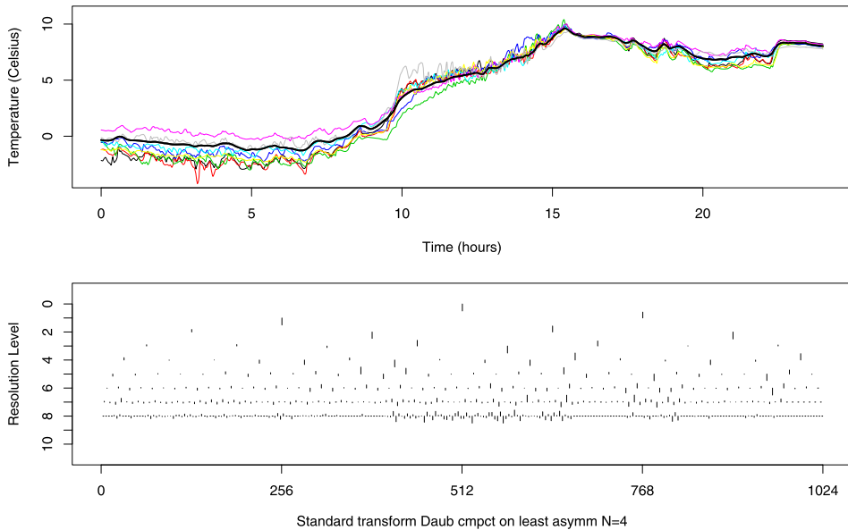
Figure 6 Application of the hierarchical model to the SensorScope data. Top: reconstruction after applying the hierarchical model with a mixture for the error variance; the dark line represents the global curve; bottom: corresponding estimates of the wavelet coefficients \zeta_{jk} .
